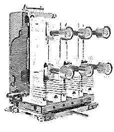
Example: Circuit breaker on withdrawable part with contact arms and contacts
