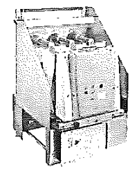
Example: Circuit breaker with withdrawable module and earthing switch
