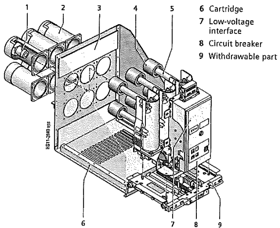
Withdrawable module 3AE5
