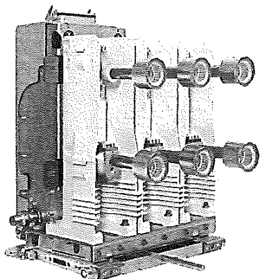
SION vacuum circuit breaker on withdrawable part – with contacts
