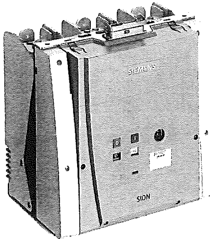
3AE1 vacuum circuit breaker as fixed-mounted version
